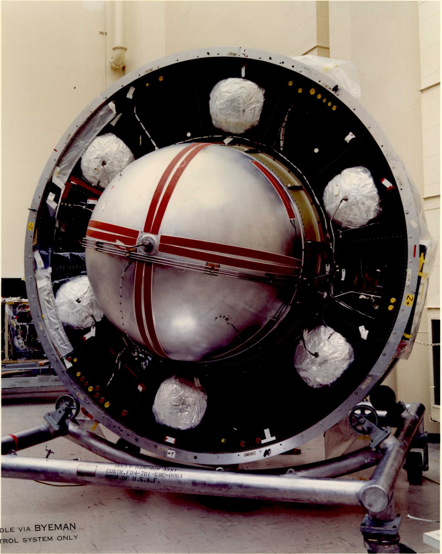
FIRST FLIGHT ORBIT ADJUST MODULE/REACTION CONTROL MODULE (LOOKING AFT)
