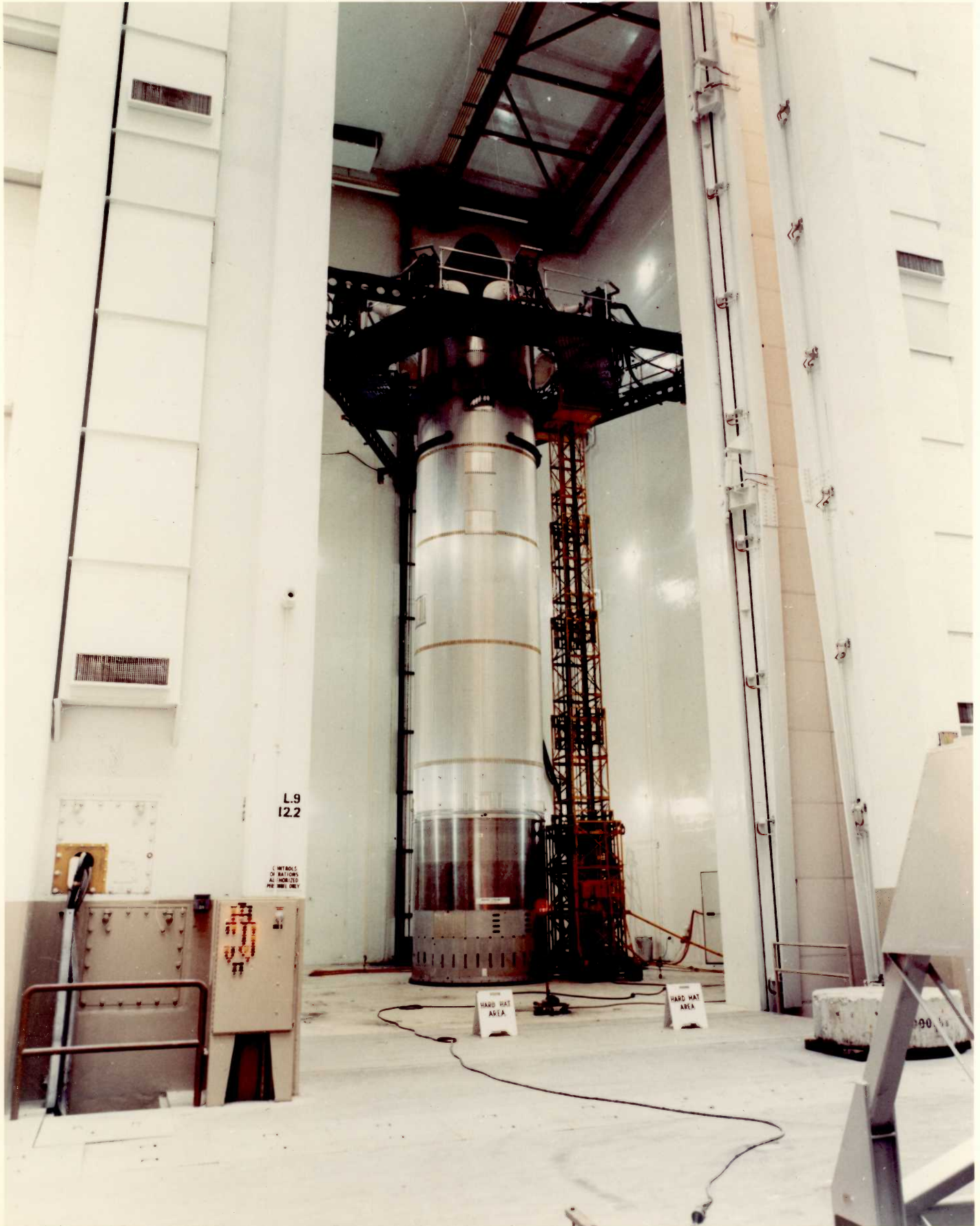
SHROUD AND TEST BASE IN ACOUSTIC CHAMBER
