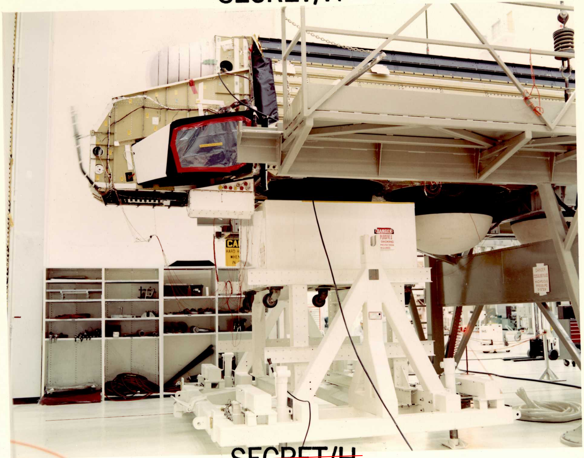
SV-5 Forward section with mapping camera module
