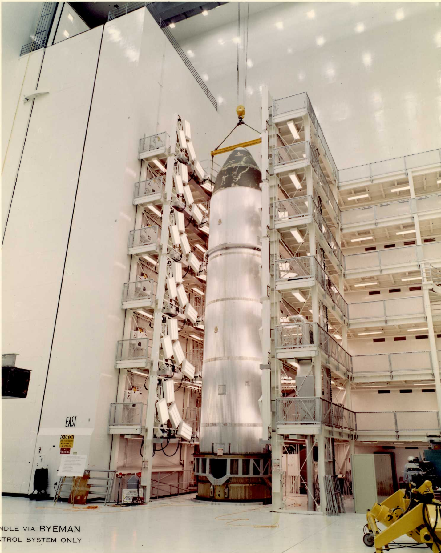
SYSTEM QUALIFICATION VEHICLE IN VIS 1 AND 2 WITH PLATFORMS RAISED
