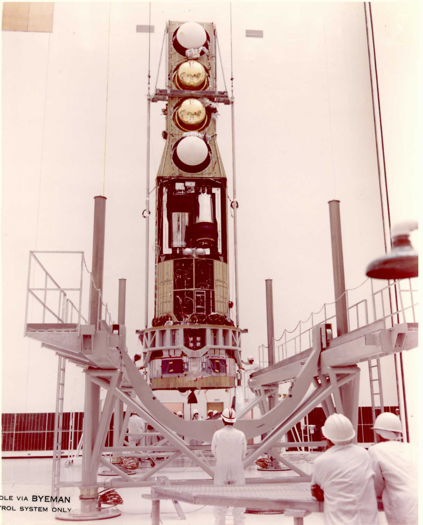
SYSTEM QUALIFICATION VEHICLE LOWERED INTO "A" FRAME OF HANDLING EQUIPMENT
