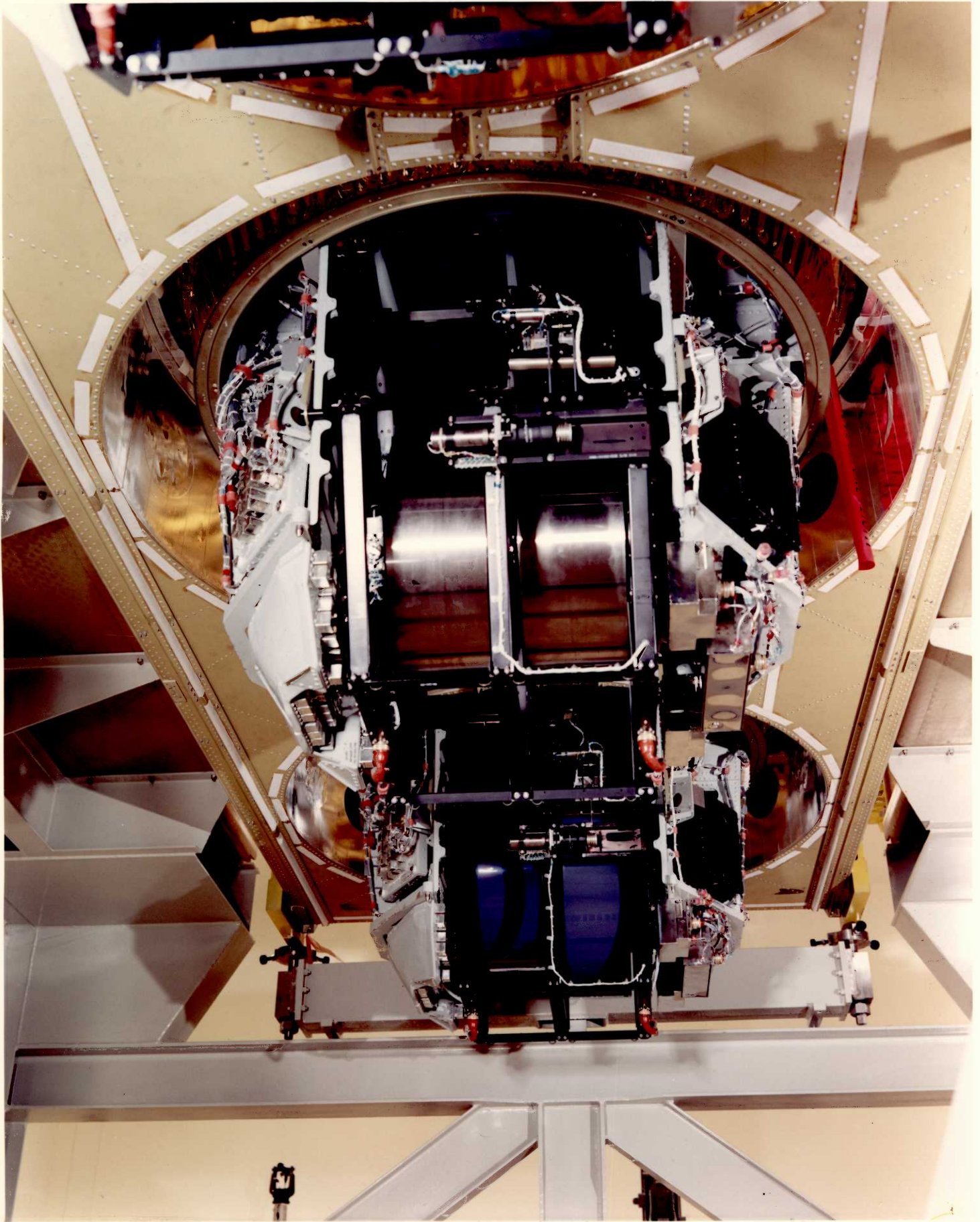
HANDLE VIA BYEMAN CONTROL SYSTEM ONLY VIEW OF RECOVERY VEHICLE UNIT TAKE-UP REELS
