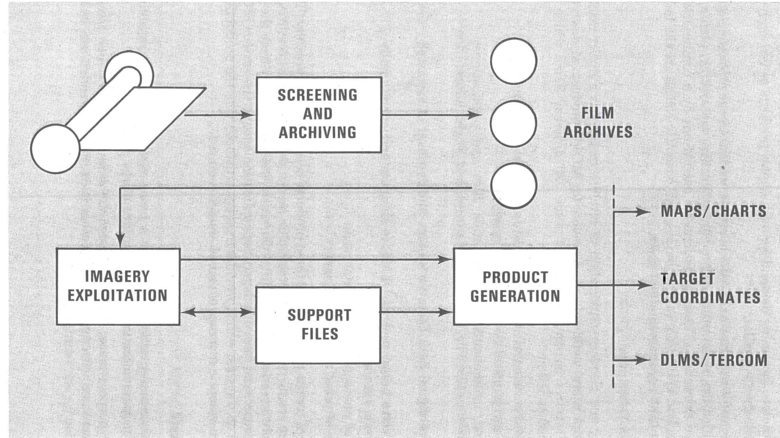
Figure 4-18. DMA MC&G Production Overview
