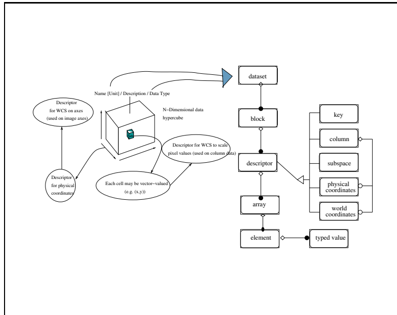
Figure 4: Conceptual structure of the CDM
