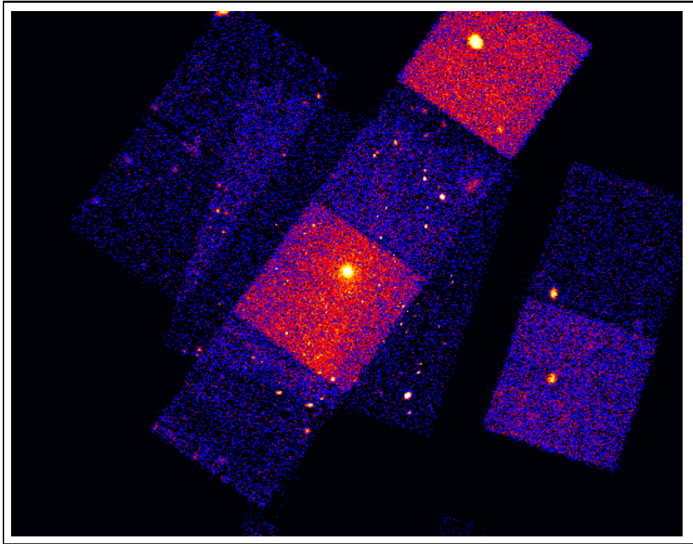
Figure 3: Three merged Chandra observations showing point sources in the nearby galaxy M33
