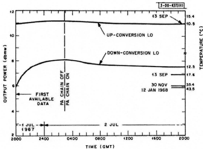
Fig. 13. Transponder local oscillators, turn-on and heating effects.
