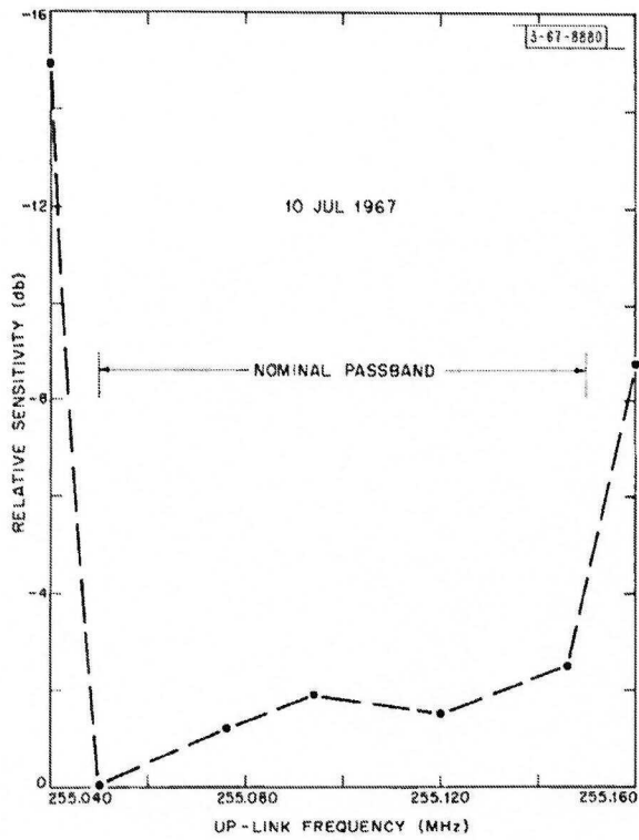
Fig. 20. In-orbit transponder sensitivity, narrowband (100-kHz) mode.
