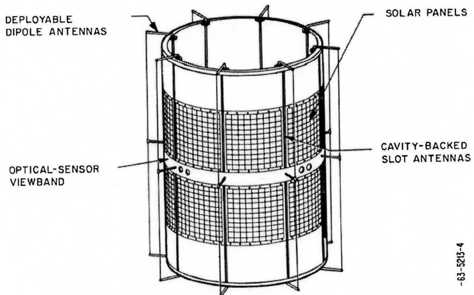
Fig. 2. LES-5 configuration.
