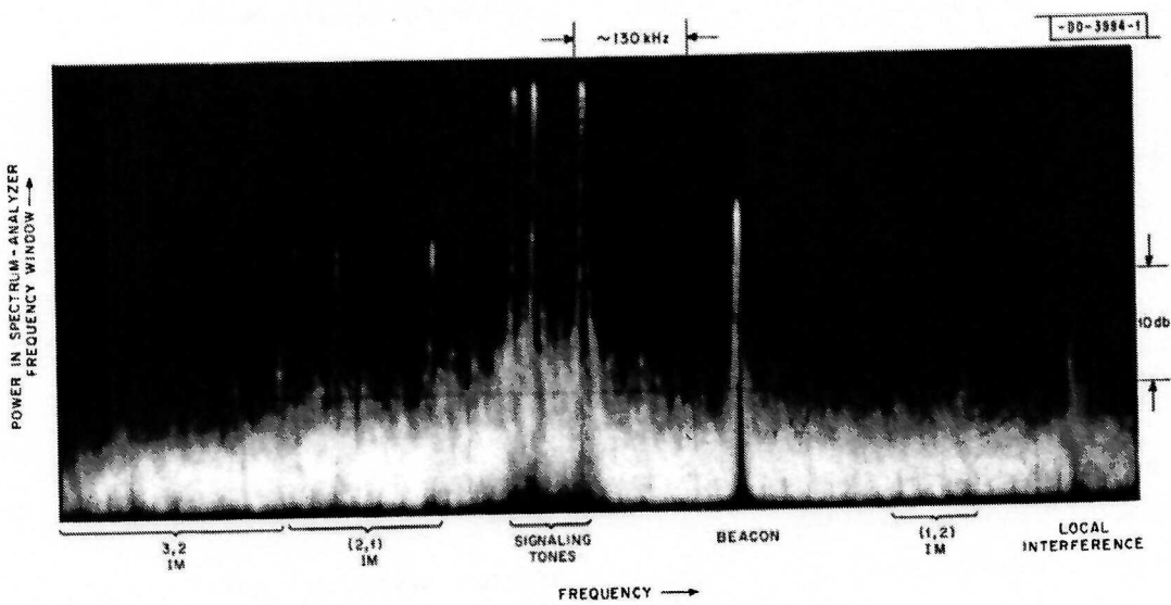
Fig. 28. Down-link signals III: Three-pair FSK tones through transponder, narrowband mode.
