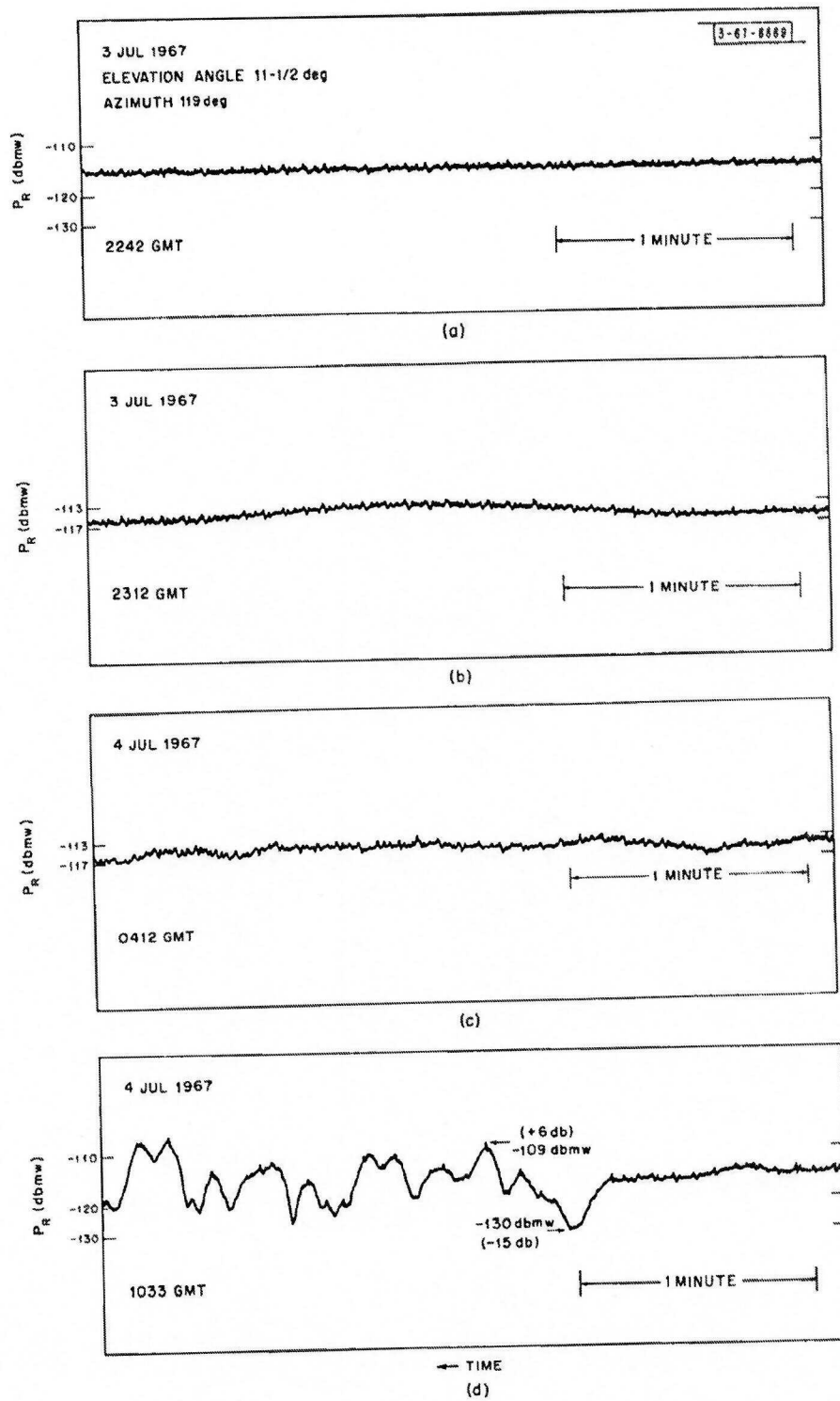
Fig. 35. Example of fading via the beacon: (a) steady signals, (b) slight fading, (c) more jittering fading and (d) severe fading.
