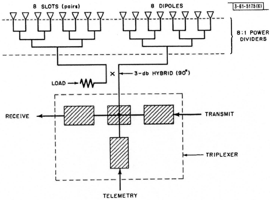
Fig. 6. Antenna feed network.
