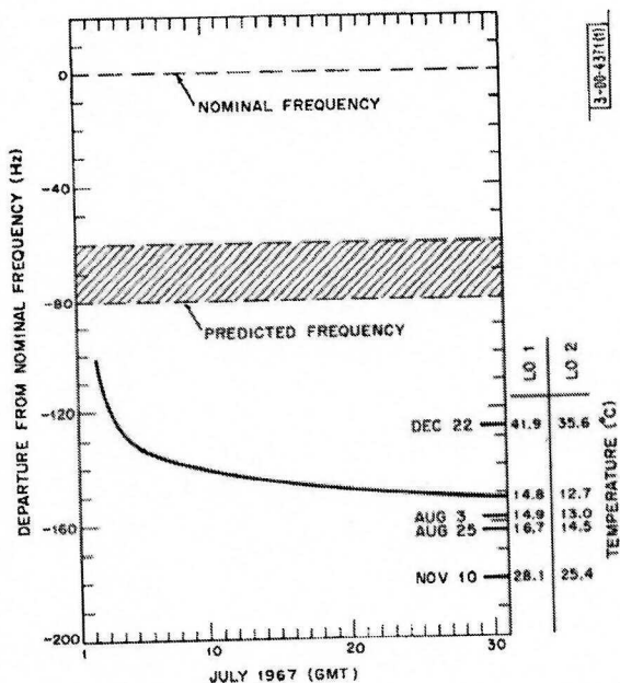
Fig. 15. Transponder frequency translation, turn-on and heating effects.
