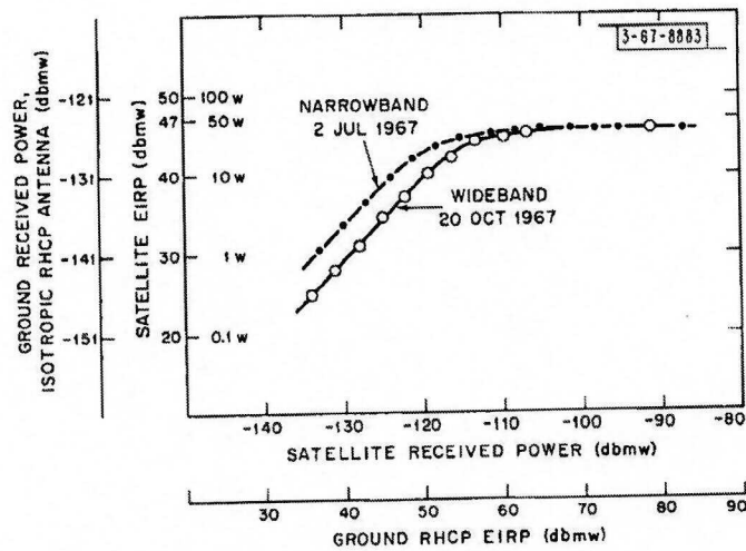
Fig. 23. Transfer curve.
