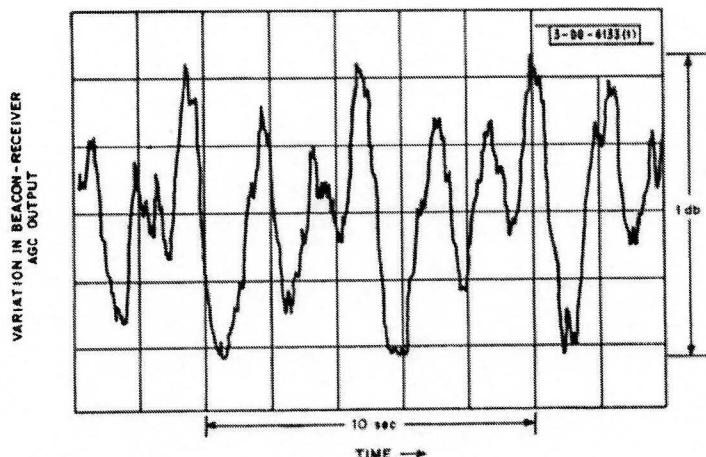
Fig. 11. Spin-modulation effects.
