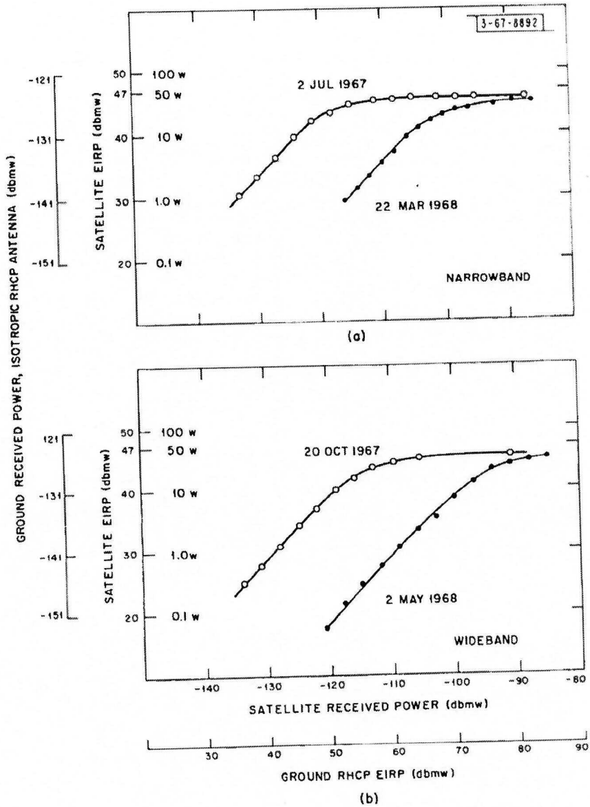
Fig. 38. Transfer curves: (a) narrowband, (b) wideband.
