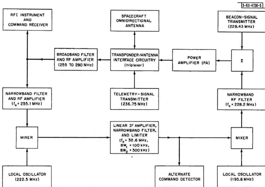
Fig. 4. LES-5 transponder and communications-associated equipments.
