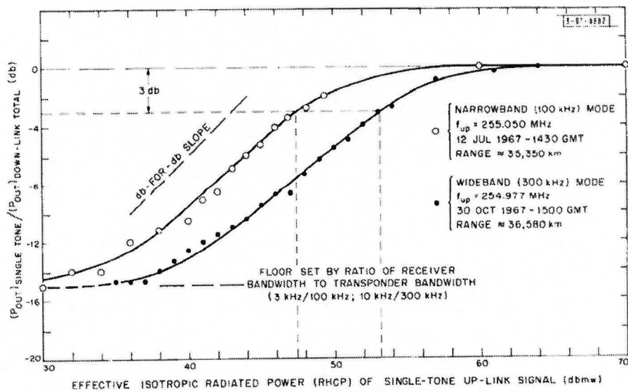
Fig. 22. In-orbit transponder limiting characteristics.
