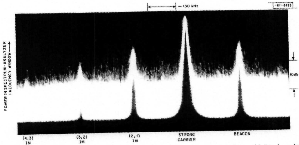
Fig. 30. Down-link signals V: Single strong tone through transponder, wideband mode.
