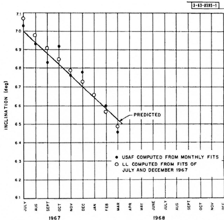
Fig. 5. Inclination variation.
