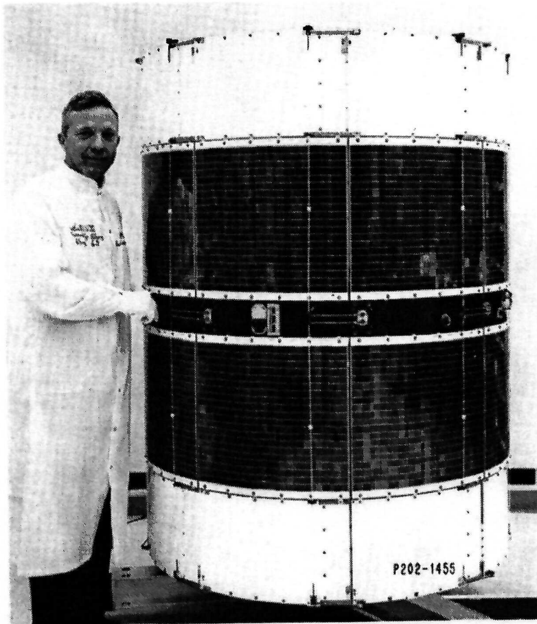
Fig. 1. LES-5 flight spacecraft.
