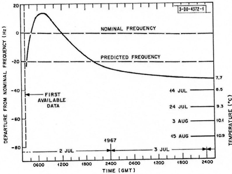
Fig. 33. Beacon-carrier-frequency turn-on and heating effects.
