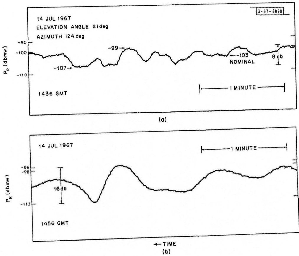
Fig. 36. Examples of fading via the transponder tone.
